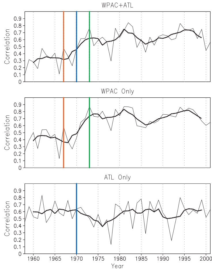
Figure 2. Correlation between 6-h BT and ERA40 Mean winds. Solid vertical line is the average R value calculated each year with the 5-year unweighted running mean (vertical dotted). The red/green (blue) lines indicate the endpoints of the respective WPAC (ATL) wind correction periods in E05.
