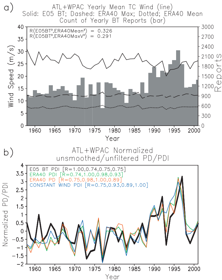
Figure 1. For all 1958–2001 NATL and WPAC TCs: (a) Mean yearly winds for BT, ERA40Mean, and ERA40Max (lines) with number of yearly BT reports in the background bar chart. Correlations are between the respective annual-mean cubed wind quantities. (b) PD/PDI normalized according to each time series individual mean and standard deviation. The line colors are described in the legend along with respective R values in matrix for comparison.
