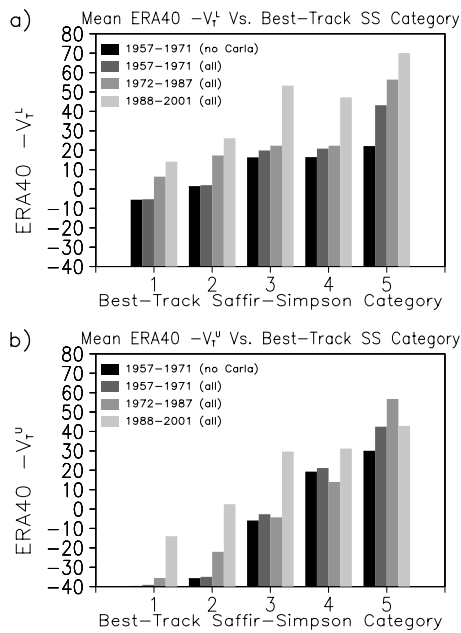
Figure 2. (a) Comparison of the mean -V_T^L for all best track hurricanes within the ERA40 data. Here the data was divided into three equal-length groups based on the relative amount of satellite data assimilated. Note that the first tercile mean changes significantly when Carla is removed from the early period. (b) The same as Figure 2a, but for the upper tropospheric thermal wind ( -V_T^U ).
