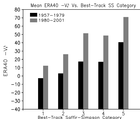
Figure 1. Comparison of the mean -V_T^L for all best track hurricanes within the ERA40 data.
