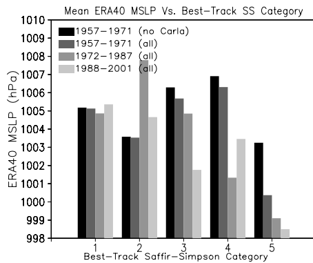
Figure 3. As in Figure 2a, except using MSLP instead of -V_T^L .
